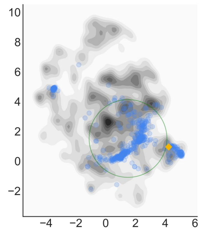
sleeping beauties
