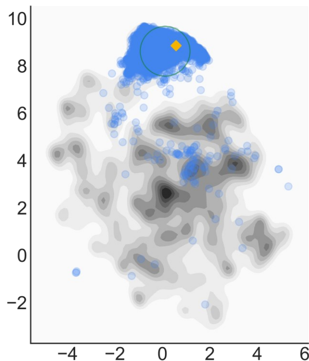
high-cited
