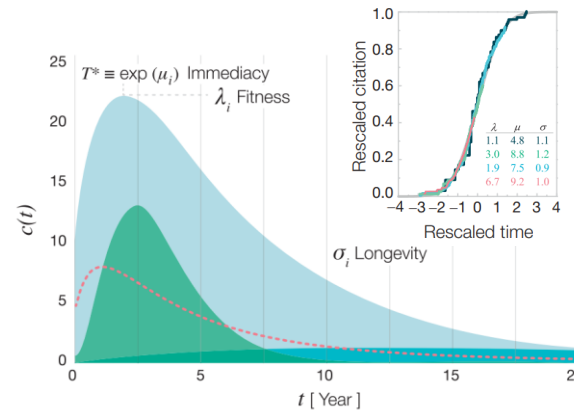
Quantifiable patterns
