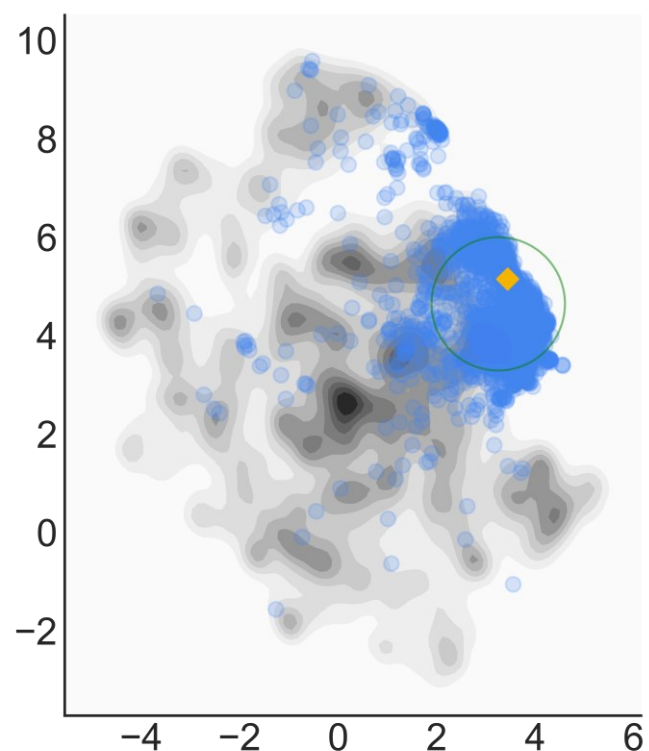
disruptive
